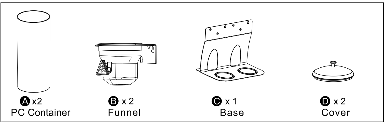
Diagram 6 - 861.348 Part List
