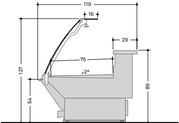
EC 550 S-CONCEPT
