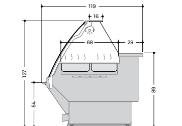
EC 450 H-COMBI
