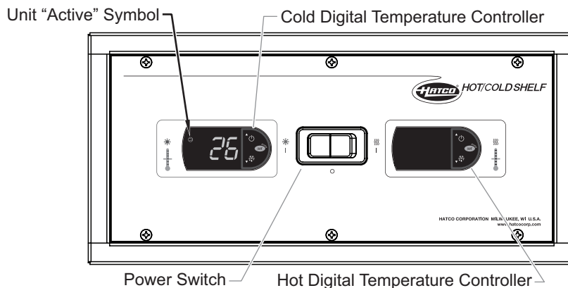
Remote Hot/Cold Shelf Control Box (shown operating in COLD Mode)
