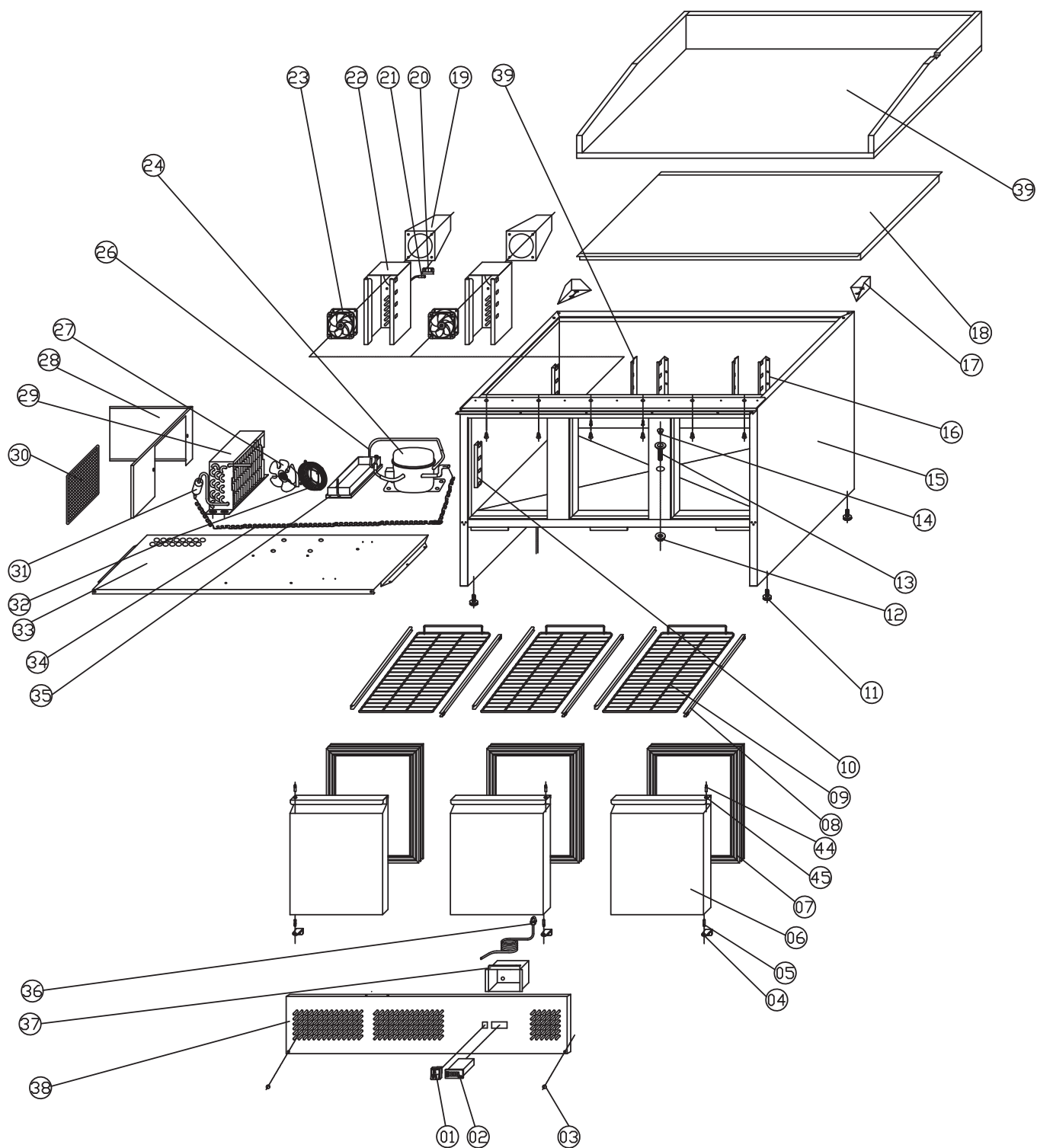
EXPLODE OF S903PZ
