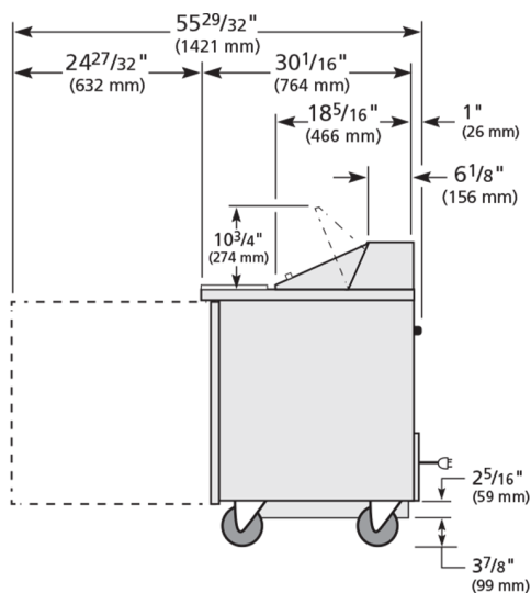
RIGHT VIEW
