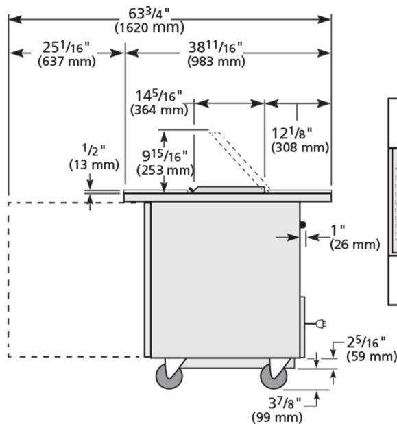
RIGHT VIEW
