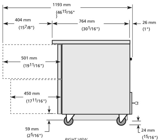
RIGHT VIEW
